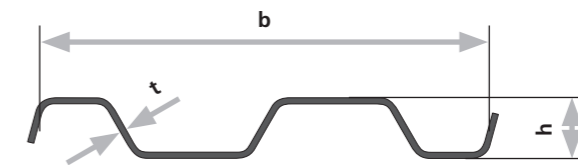
KD 6/8 sheet piles
